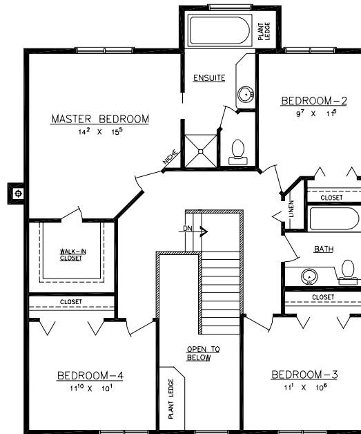
SECOND FLOOR AREA = 1030 S.F.
